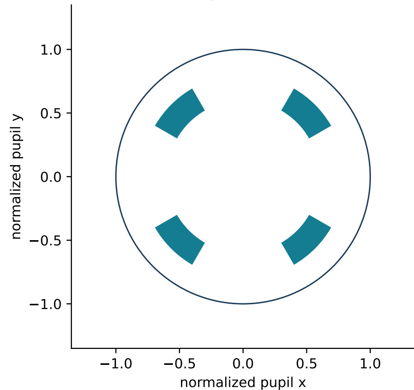
Idealized quasar illumination
